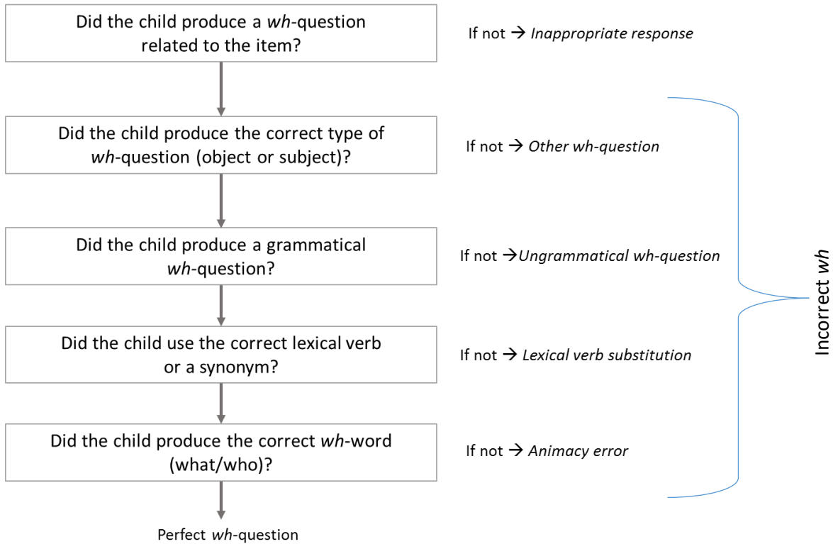
Figure 3: Step-by-step coding procedure
